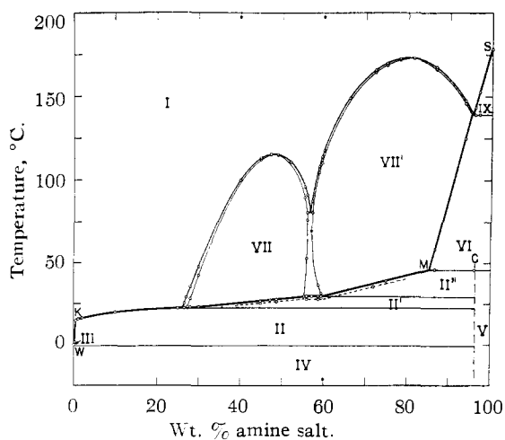
Fig. 2.—The system methyl-dodecylammonium chloride-water.
